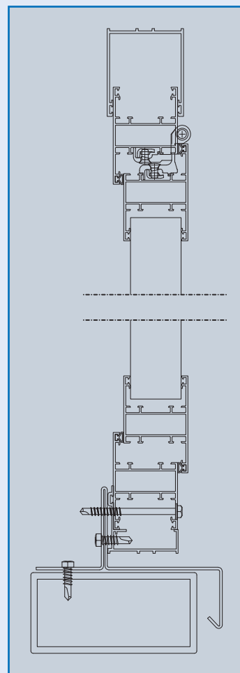
Typical window solution
