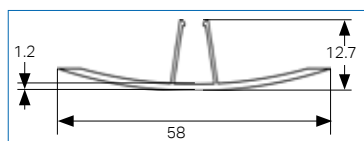
Bottom Side Free Shape
